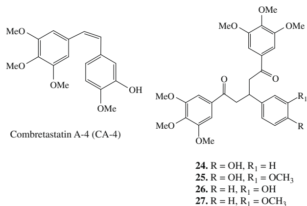
Figure 1. The Michael adducts ( 24–27 ) obtained from the Claisen Schmidt condensation between 3,4,5-trimethoxyacetophenone and corresponding benzaldehyde under reflux.
