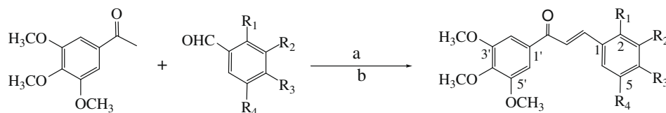
Scheme 1. General synthetic route for the synthesis of 3',4',5'-trimethoxychalcone analogues.
